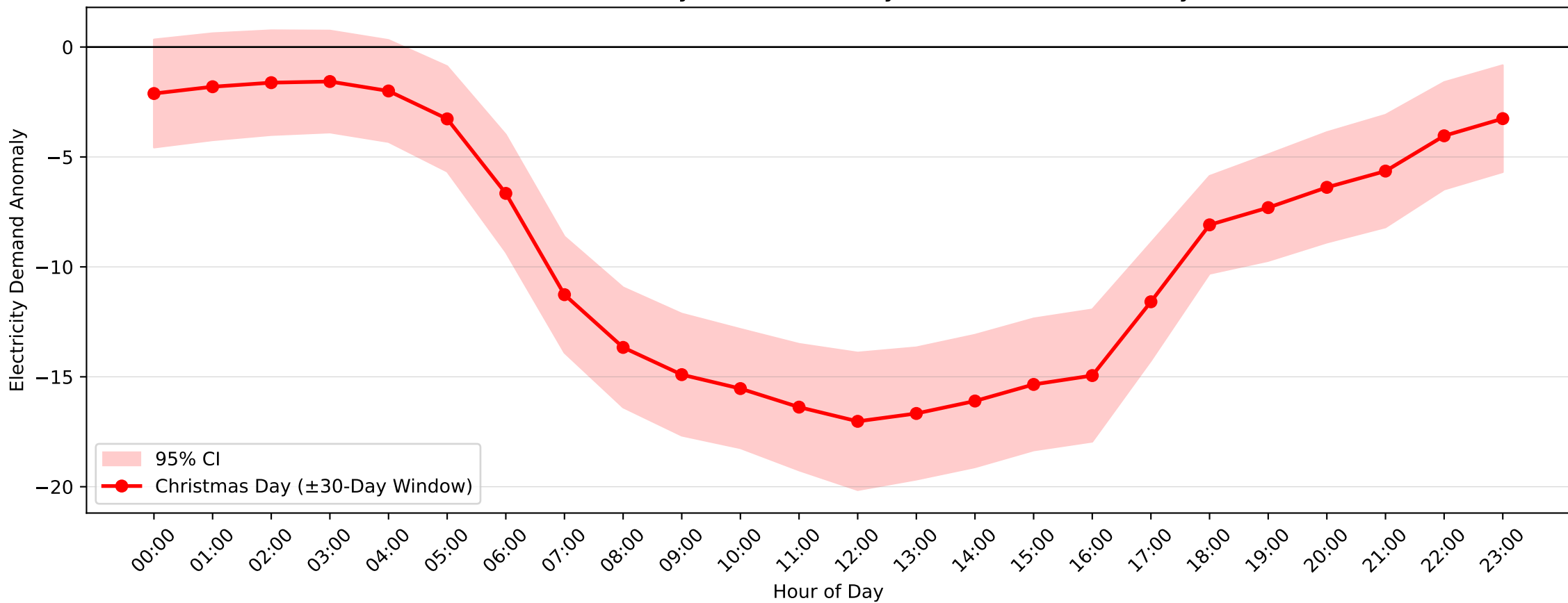
Gore Hill Demand Anomaly: Christmas Day (2004-2017, \pm 30 -Day Window)
